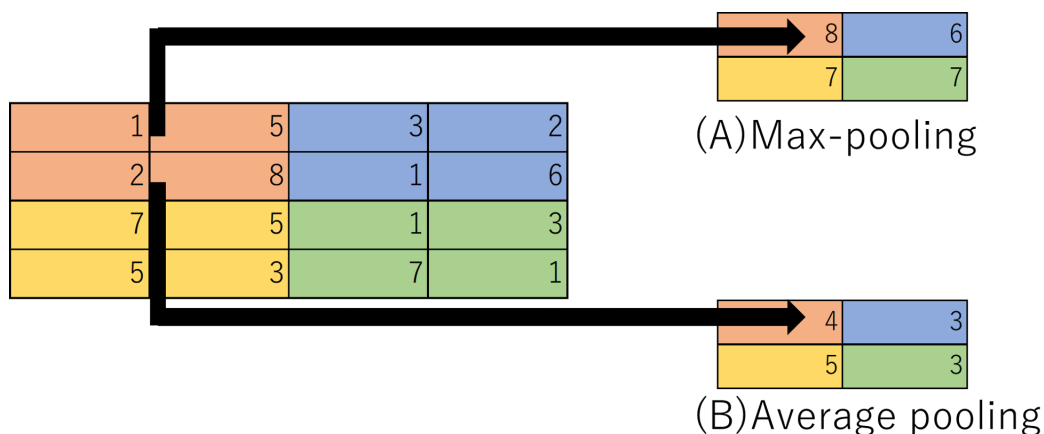
Figure 3.3: Pooling.
