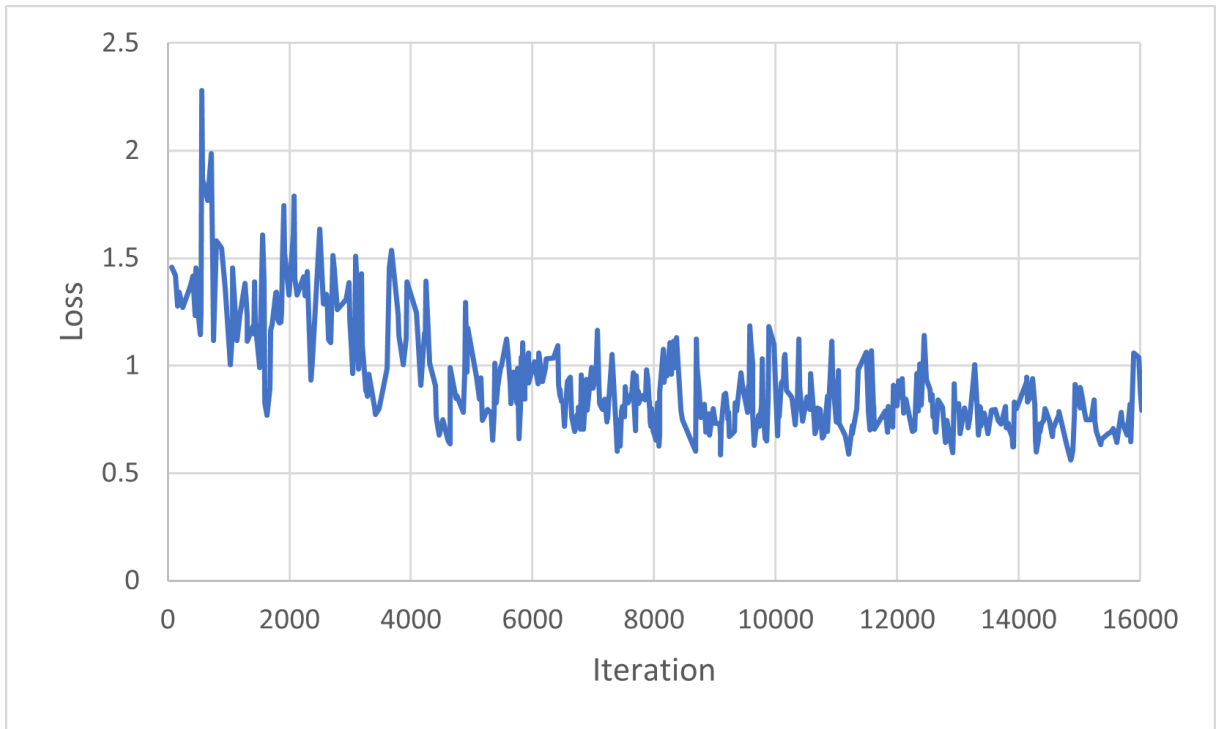
Figure 6.4: Domain classification loss of discriminator in previous experiment.
