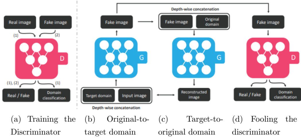
Figure 5.2: Train of discriminator and generator.[9]
