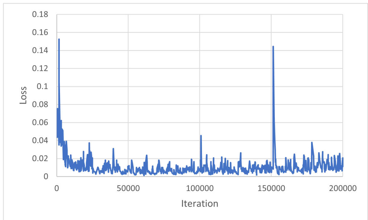
Figure 6.15: Gradient p enalty loss.
