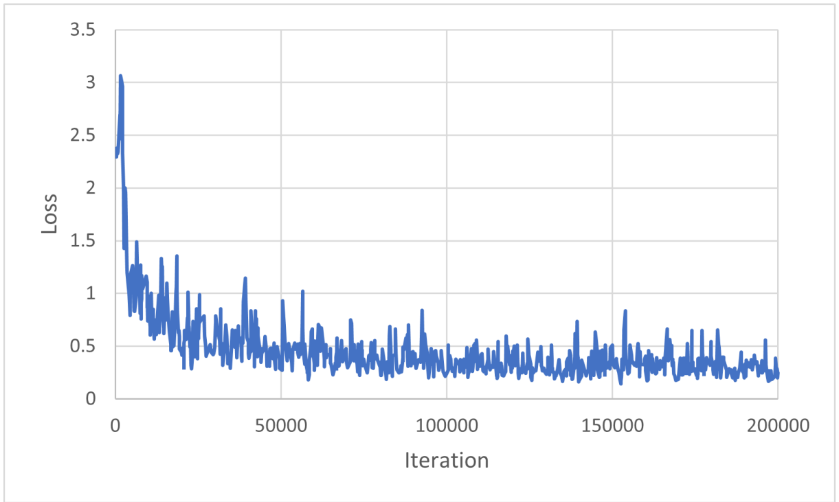
Figure 5.8: Domain classification loss of generator.
