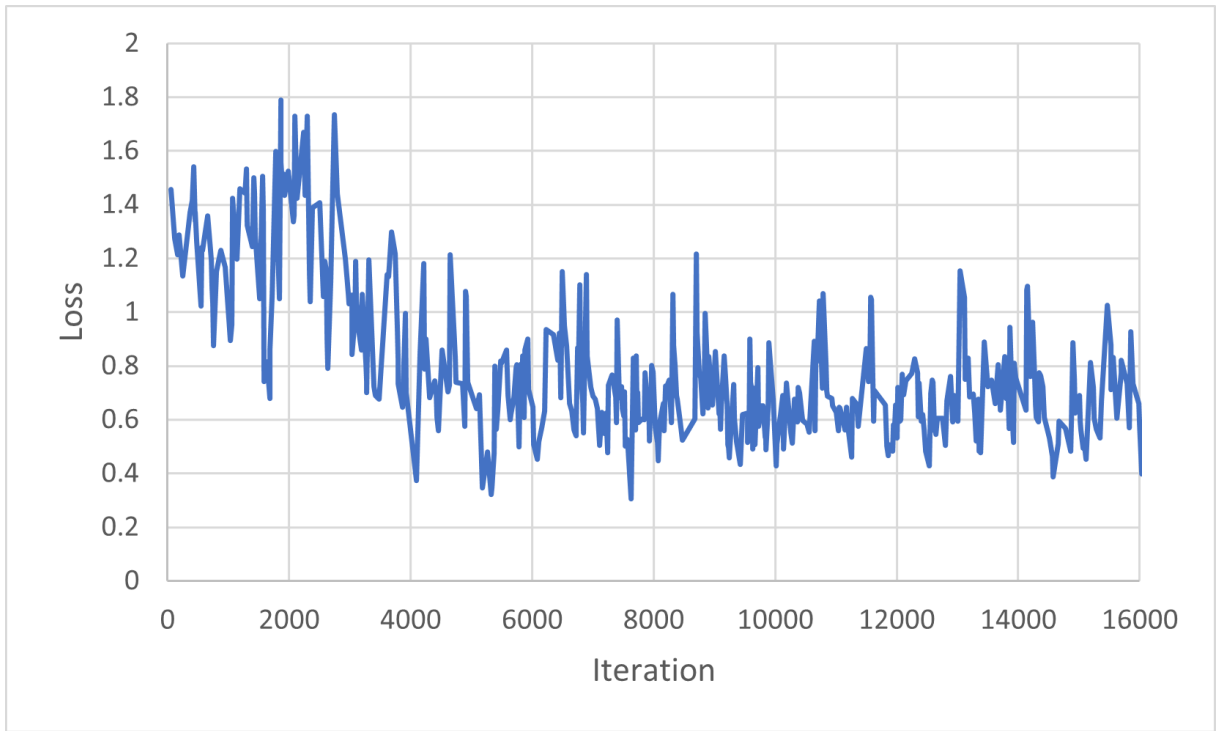
Figure 6.8: Domain classification loss of generator in previous experiment.
