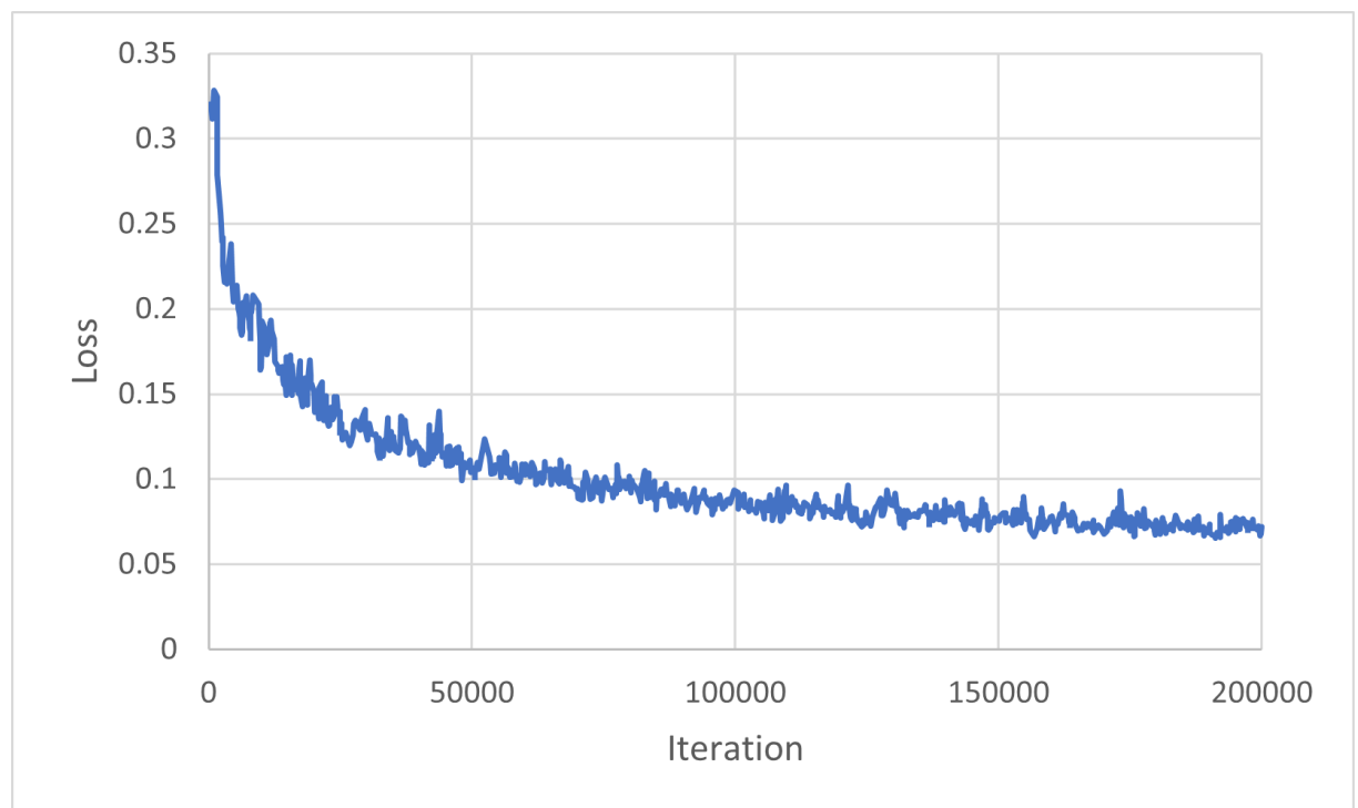
Figure 6.18: Reconstruction loss of generator.
