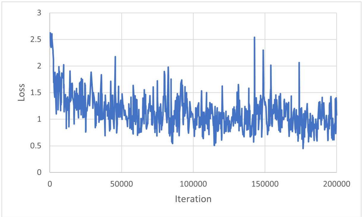
Figure 5.4: Domain classification loss of discriminator.
