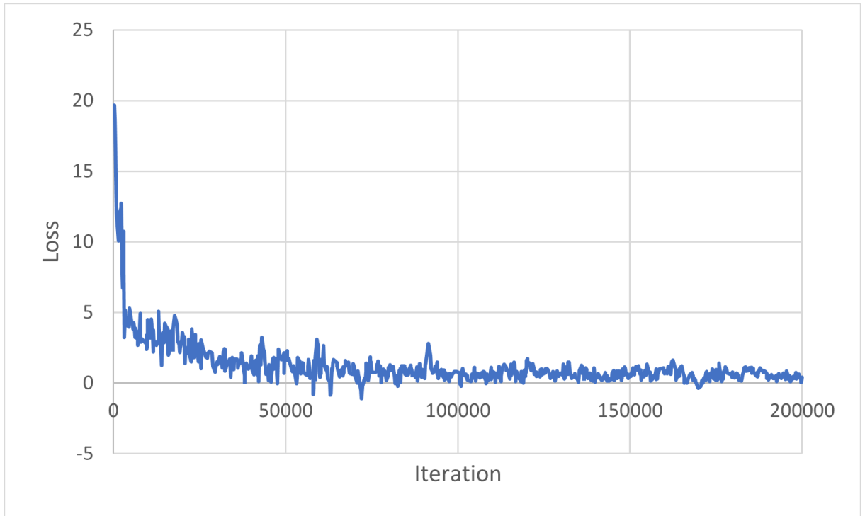
Figure 5.5: Adversarial loss on fake images of discriminator.
