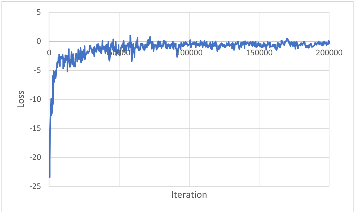
Figure 5.9: Adversarial loss of generator.
