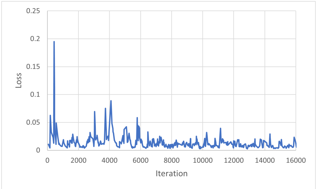
Figure 6.7: Gradient p enalty loss in previous experiment.
