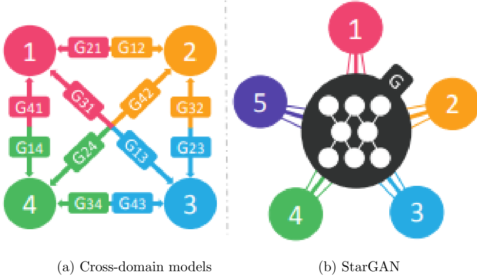
Figure 5.1: Conversion between multiple domains of each model.[9]
