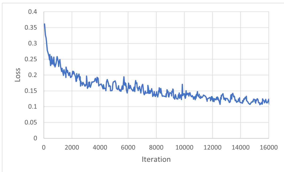
Figure 6.10: Reconstruction loss of generator in previous experiment.
