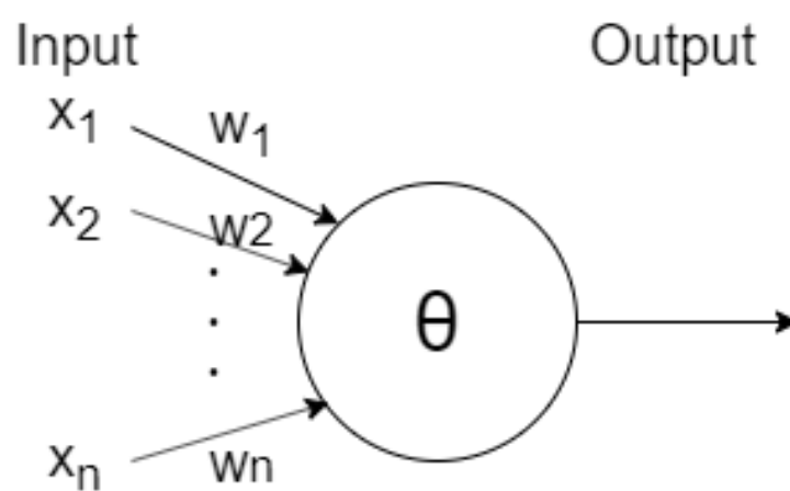
Figure 2.2: Neuron model.
