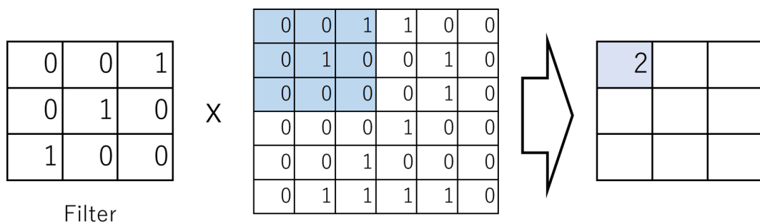
Figure 3.2: Convolution.
