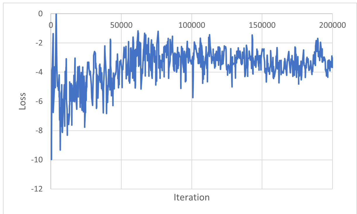
Figure 6.14: Adversarial loss on real images of discriminator.
