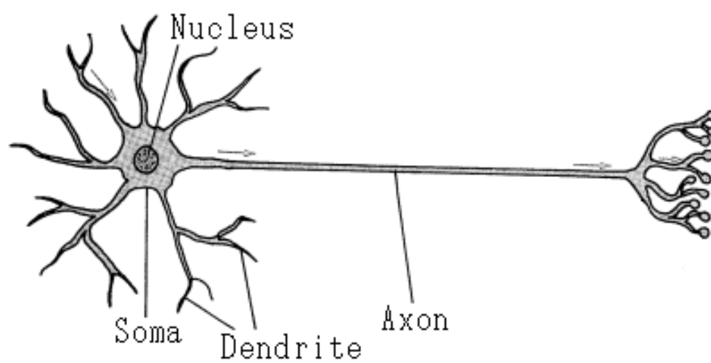
Figure 2.1: Neuron.[1]
