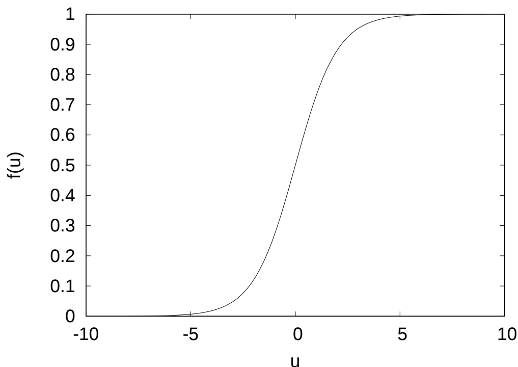
Figure 2.3: Sigmoid function.
