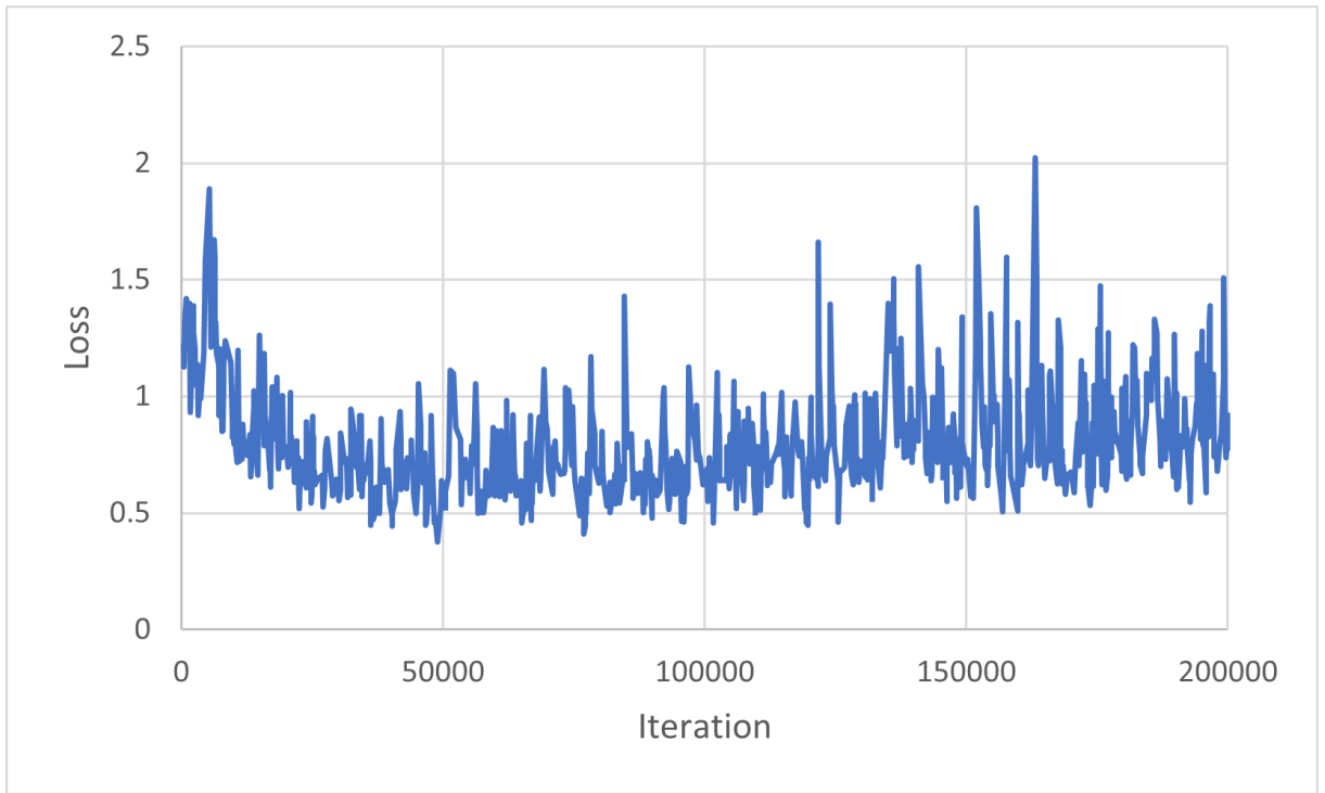
Figure 6.16: Domain classification loss of generator.
